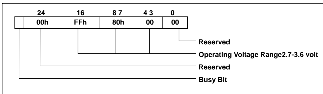
OCR Structure
