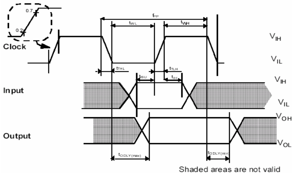
Timing Diagram Data Input. Output Referenced to Clock
