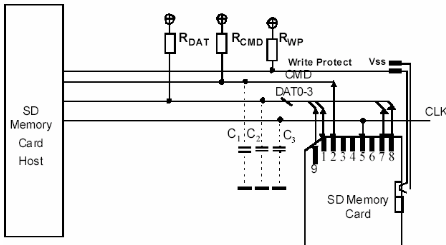
Bus Circuitry Diagram
