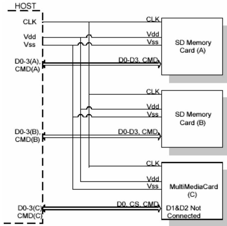
SD Card System Bus Topology
